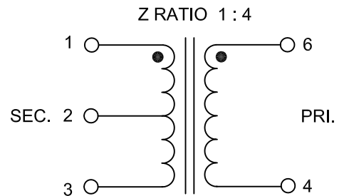
SCHEMATIC
