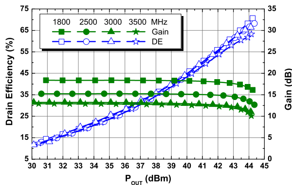
Figure 10 - Typical CW Performance over frequency in Load-Pull
