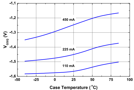
Figure 15 - Quiescent Gate Voltage ( V_{GSQ} ) Required to Maintain I_{DQ} as a Function of Case Temperature, V_{DS} = 28V
