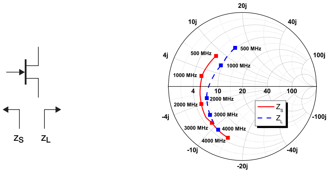
Figure 3 - Optimum Impedances for CW Performance, V_{DS} = 28V
