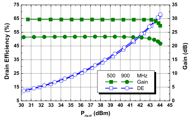
Figure 2 - Typical CW Performance 1 over frequency in Load-Pull, V_{DS} = 28V , I_{DQ} = 225mA
