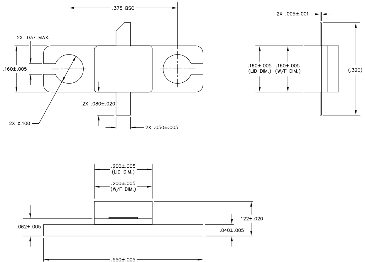
Figure 17 - AC200BM-F2 Package Dimensions and Pinout (all dimensions are in inches)
