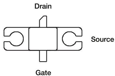
Figure 18 - Terminal Identification
