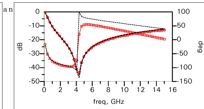
Figure 2 · Modeled S_{11} for a 4.7 pF surface mount capacitor on 14 mil-thick FR4 in a series 2-port configuration. Results are shown for an accurate, substrate-scalable model—solid line with circles (magnitude) and squares (phase)—and a simplified series L-C equivalent circuit (lines).
