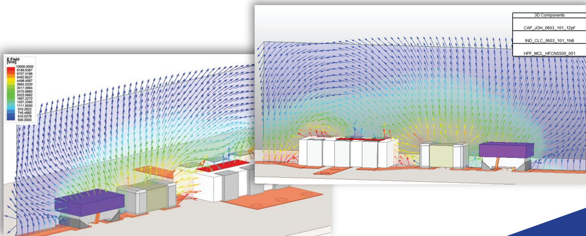
Modelithics 3D inductor, capacitor, and filter models.
