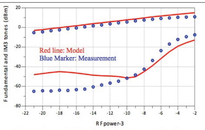
(b) P2D model simulated fundamental and IM3 tones compared to measured results.
